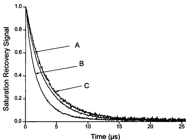
FIGURE 3 Typical saturation-recovery signal of ^{14}\text{NC16} in DMPC membranes at 27^\circ\text{C} . T_{1c} = 2.39 , 2.11 , and 2.58 \mu\text{s} in the absence of modifiers (A) or the presence of 20 mol% cholesterol (B) or 10 mol% lutein (C), respectively.
