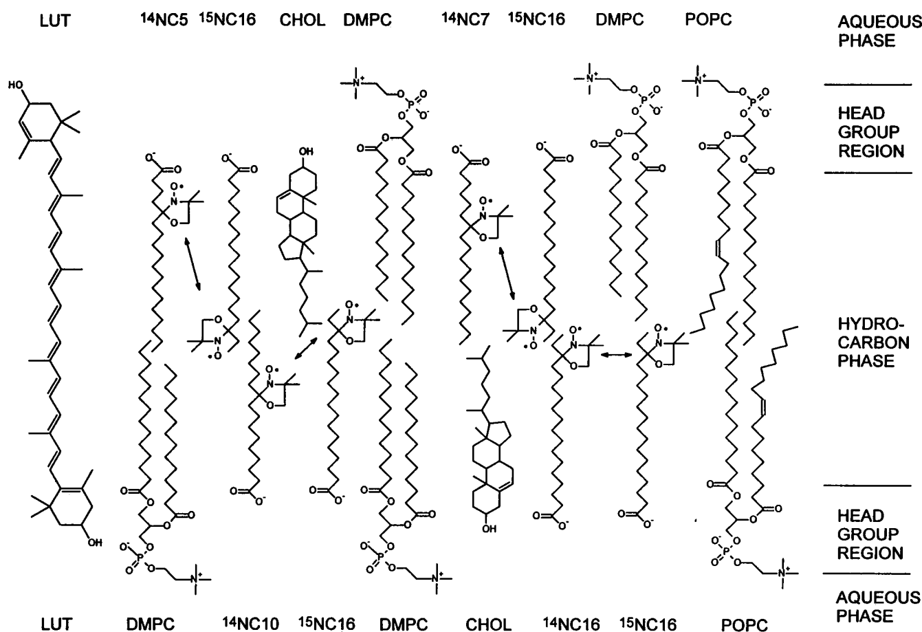
FIGURE 1 Cross-sectional drawing of the lipid bilayer including lutein, cholesterol, and spin labels. Observed collision between ^{14}\text{N} : ^{15}\text{N} spin-label pairs are indicated. DMPC and 1-palmitoyl-2-oleoyl PC (POPC) molecules are also shown. POPC represents the major component (70%) of the EYPC mixture (Seelig and Waespa-Sarčević, 1978).
