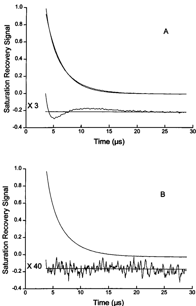
FIGURE 4 Saturation-recovery signal and curve fitting for ^{14}\text{NC10} : ^{15}\text{NC16} (0.5:0.5 mol%) in DMPC at 27^\circ\text{C} , pH 9.5. The recovery curve contains 512 data points with a resolution of 50 ns per point. Simulations and experimental saturation-recovery signals are superimposed. The differences, multiplied by a factor of 3 for single-exponential fitting (A) and by a factor of 40 for double-exponential fitting (B), are shown as the "residual" beneath the recovery curve. Each recovery signal was obtained in 2 min at 6000 accumulations/s. The time constants are 3.38 \mu\text{s} and 0.97 \mu\text{s} from the double exponential fitting.
